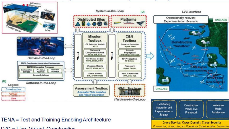
Figure 2: Distributed Experimentation Environment
